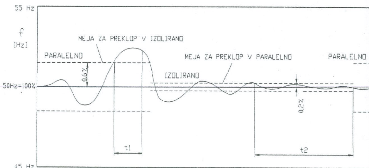
Fig 9: Parallel <=> Isolated switching
